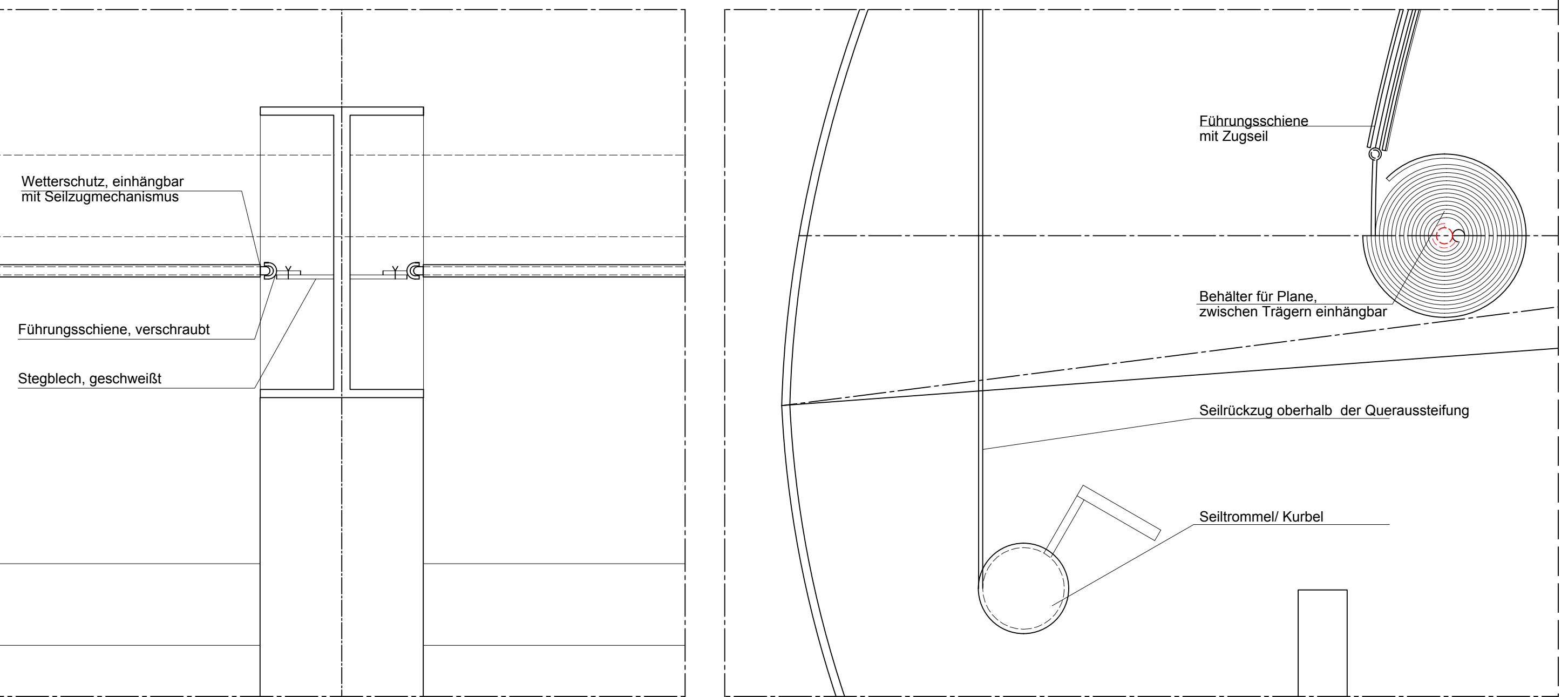
Detail 1:5
